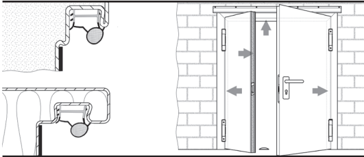
Figure C (refers to PROGET FIRE RATED and MULTIPURPOSE doors)
